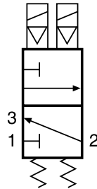
Simplified Schematic
