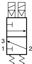
Simplified Schematic
