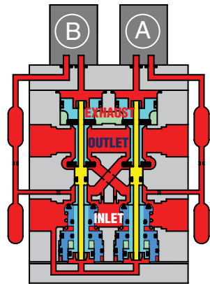
Valve actuated.
