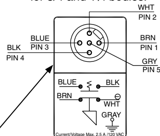
Sensing Switch Cable with 5-pin M12 Connector for 2 inch body.
