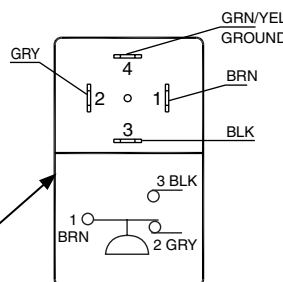
Status Indicator Cable with DIN Connector
